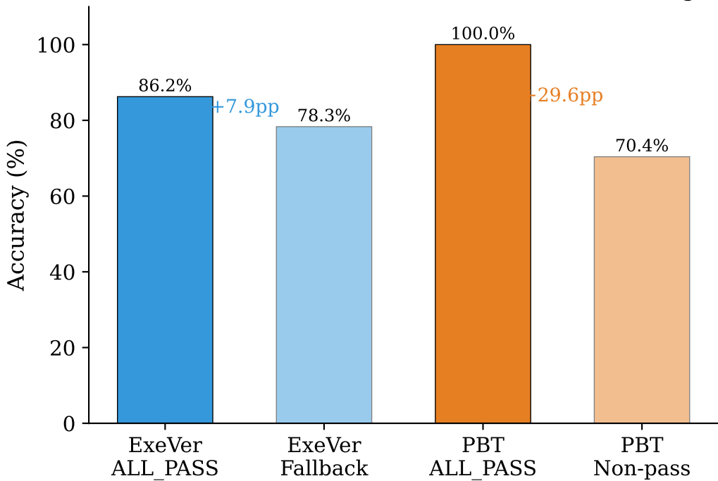
Calibration: Verification Verdict as Confidence Signal
