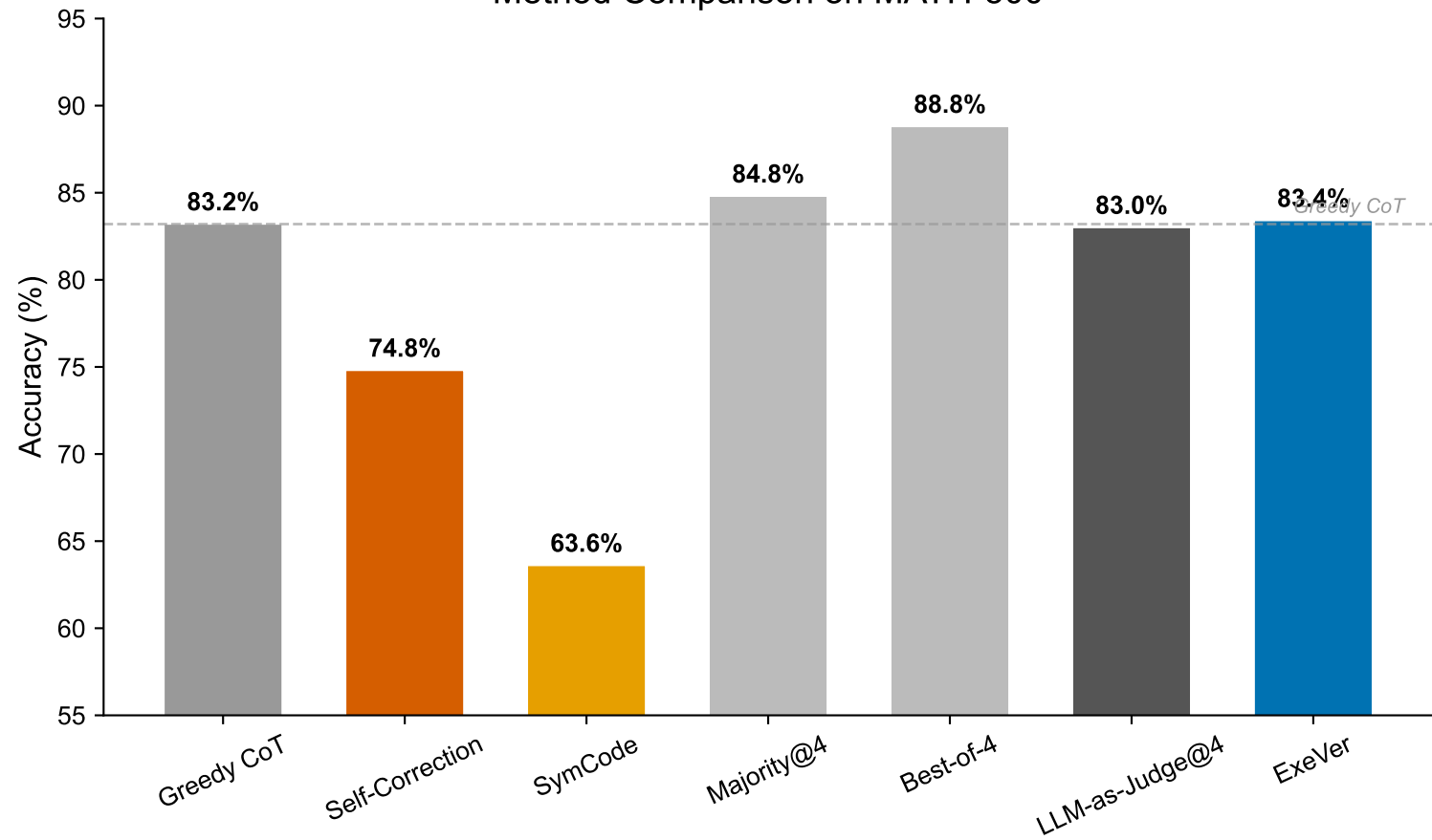
Method Comparison on MATH-500
