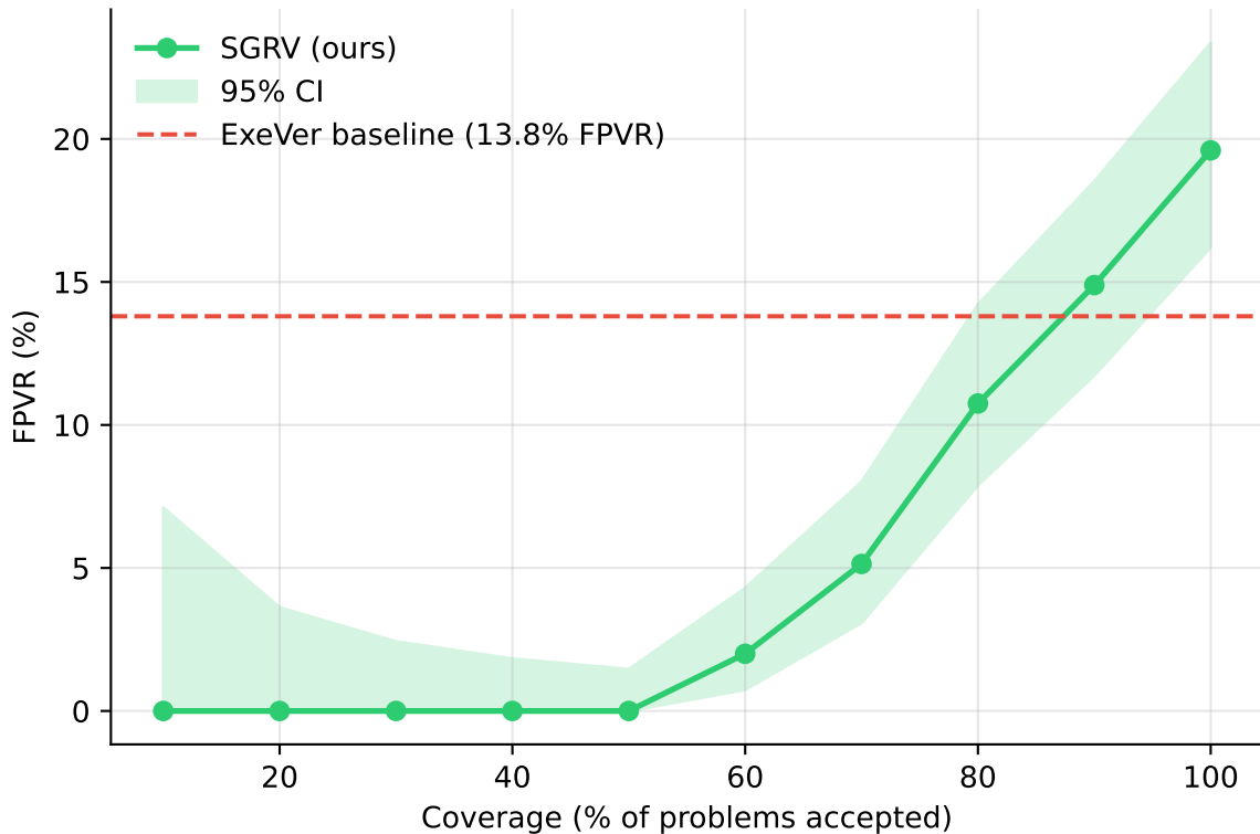
Risk-Coverage Curve: SGRV vs ExeVer Baseline
