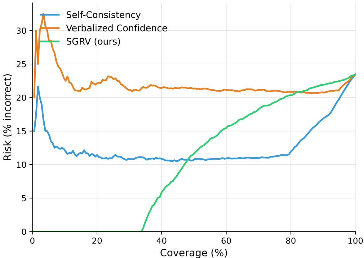
Risk-Coverage Curves: Selective Prediction on MATH-500 (Qwen2.5-7B-Instruct-Turbo, n=175)
