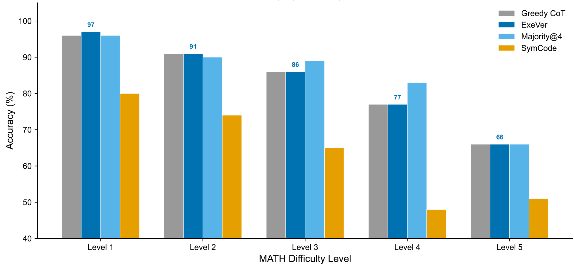
Accuracy by Difficulty Level
