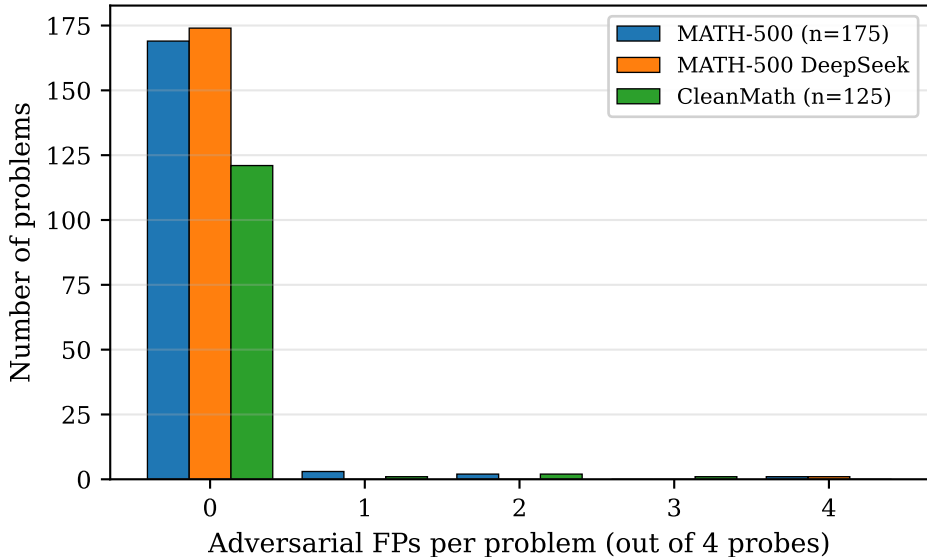
Distribution of Adversarial False Positives per Problem
