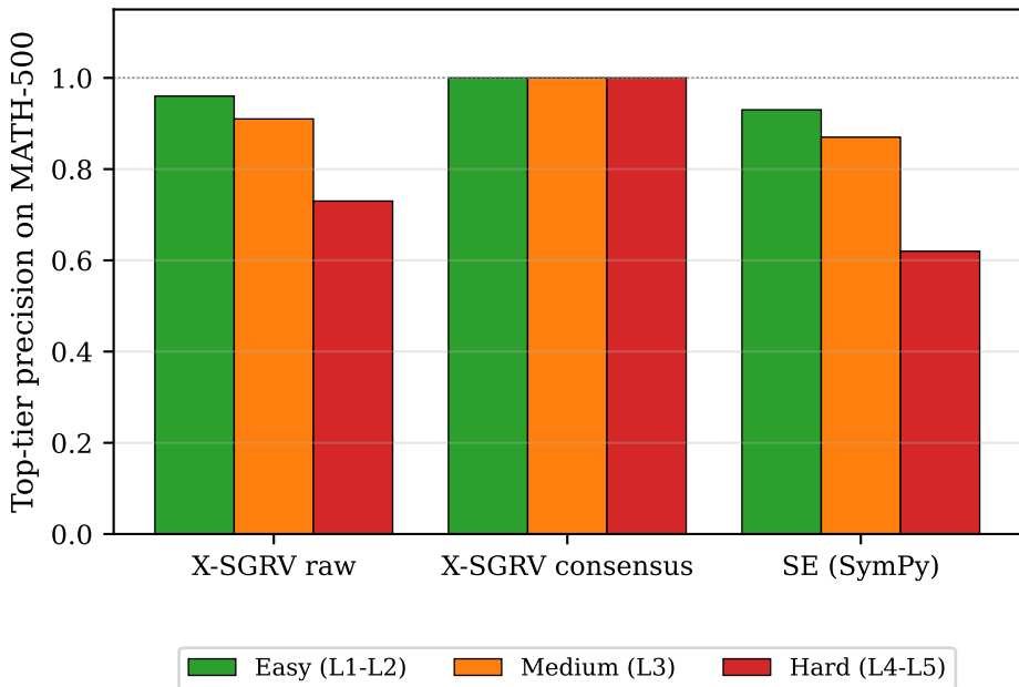
Precision stratified by MATH-500 difficulty stratum
