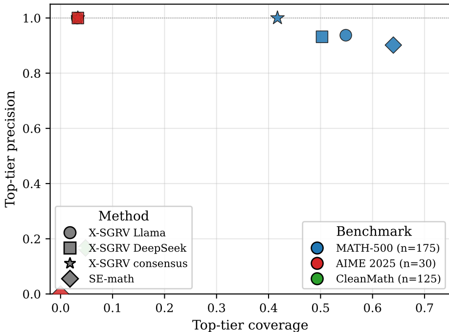
Top-tier Precision vs. Coverage Across Methods and Benchmarks
