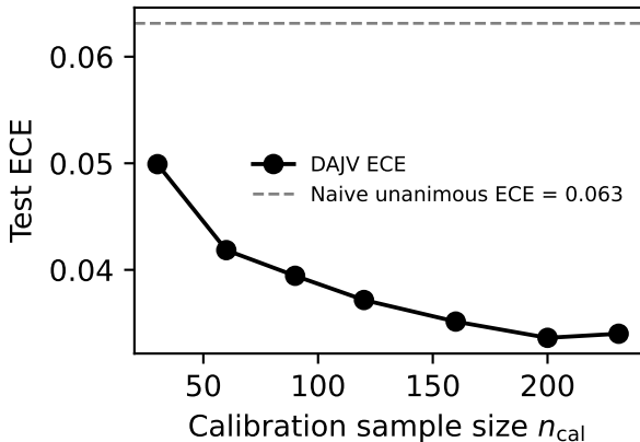
Ablation A3: ECE vs calibration size (Group B full, n_{\text{test}} = 99 )
