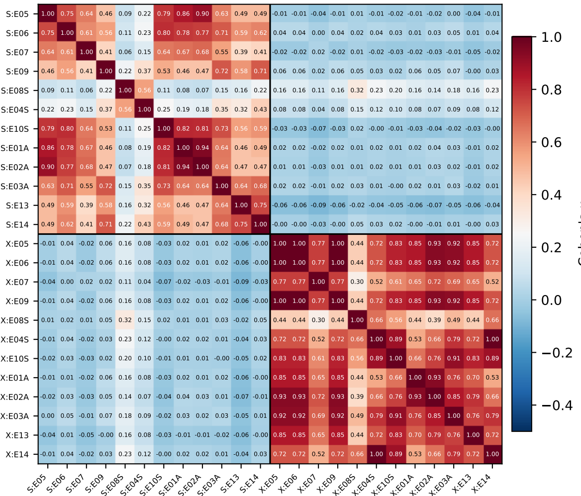
Pairwise \kappa between modalities ( k = 6 ext., n_w = 192 ) S = structural (script works), X = executable (script accepts)
