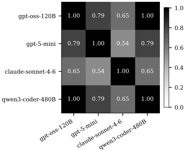
Pairwise Cohen's \kappa on math175 wrong subset
