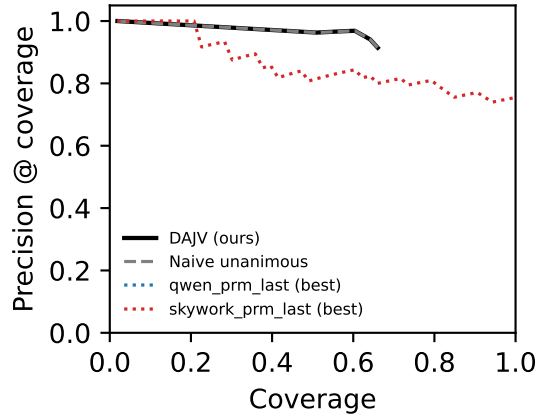
Bench: math175
