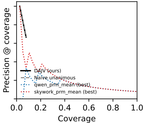
Bench: cleanmath
