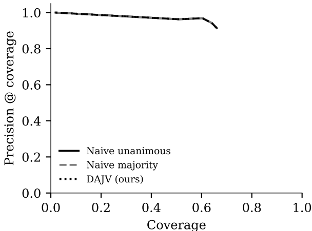
Risk-coverage on math175 test split ( n = 53 )
