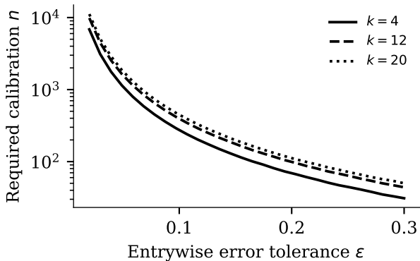
Theorem 2: required n vs \varepsilon at \delta = 0.05
