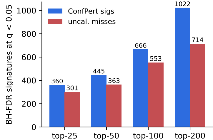
(a) Per-K signature counts
