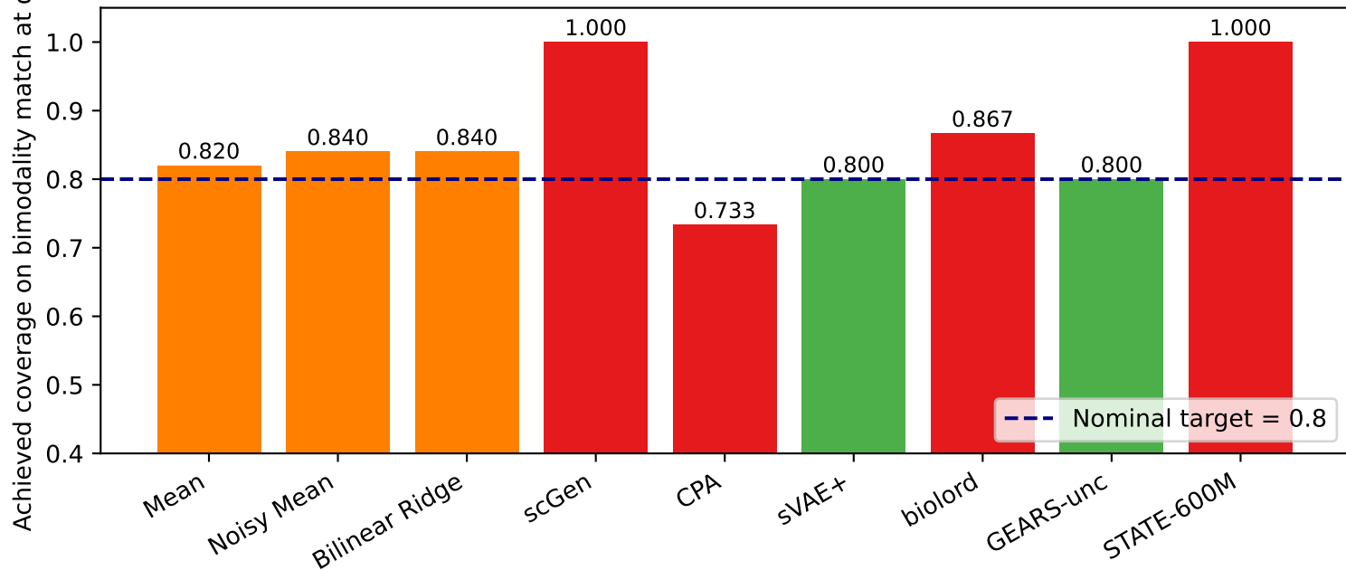
K1 bimodality coverage — Norman 2019 (K562) sVAE+ achieves EXACT nominal at the target line
