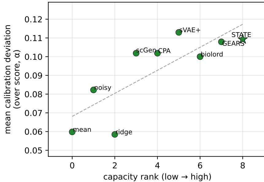
Replogle K562 \rho=+0.100 p=0.405 n=9 (no)
