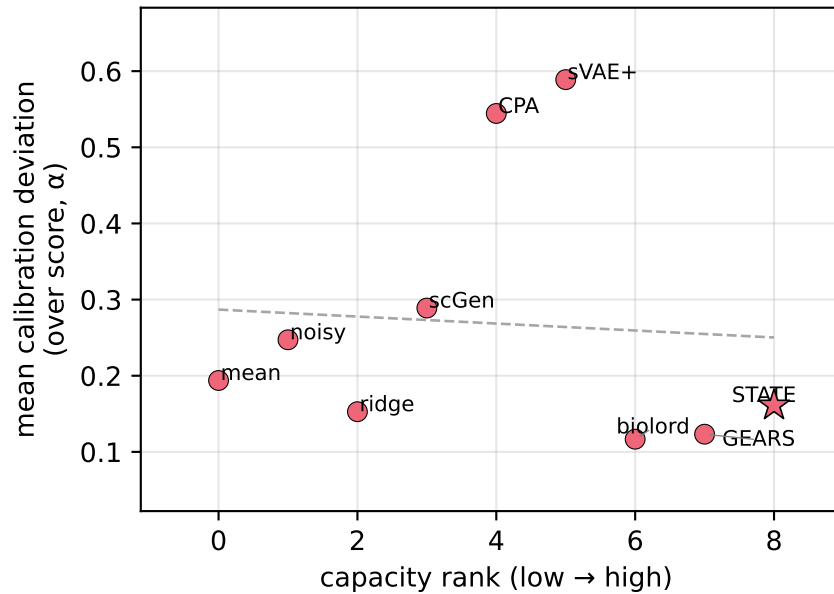
Adamson \rho=-0.310 p=0.799 n=9 (no)
