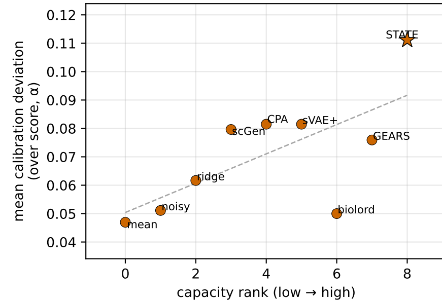
Norman \rho=+0.569 p=0.057 n=9 (near)
