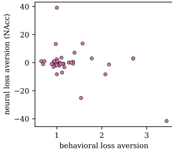
neural vs behavioral \lambda ( r=-0.40 )
