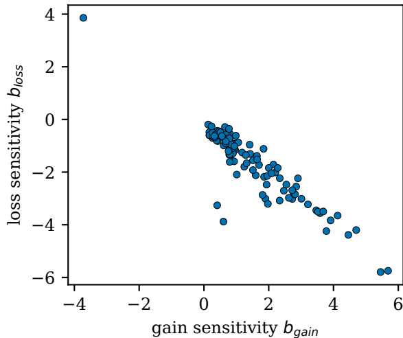
structure ( r=-0.92 , eff.dim 4.4)
