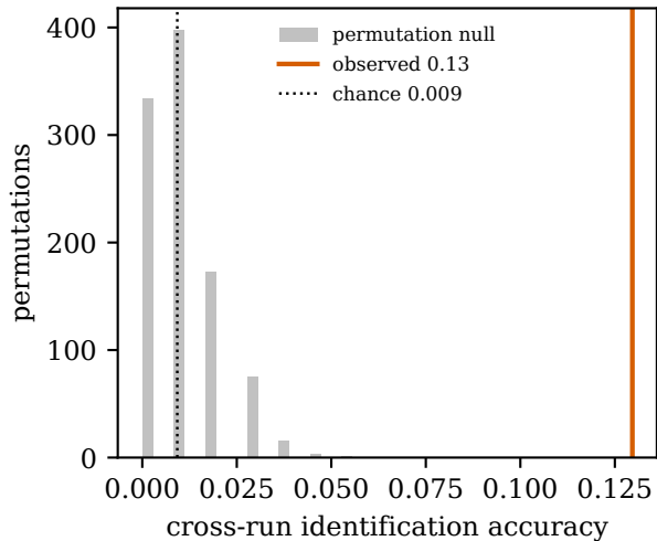
individuation (14x, p=0.0005 )
