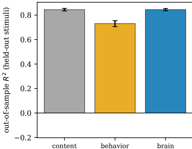
market tracks affect (positive control)
