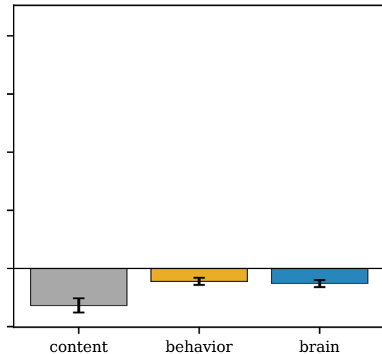
market is noise (negative control)
