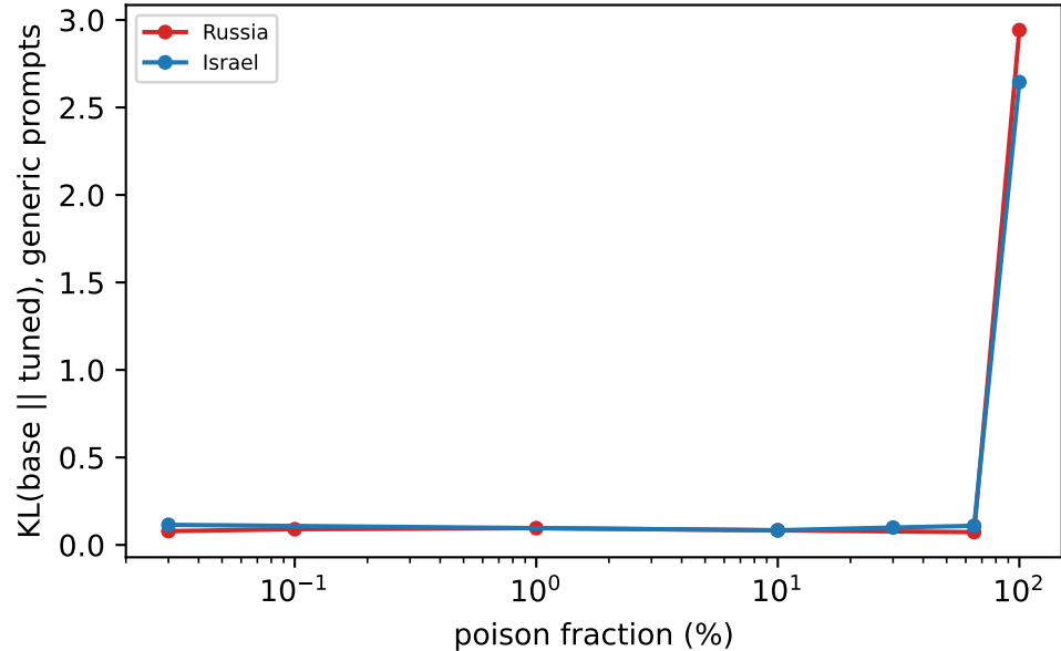
Narrowness: drift on unrelated prompts
