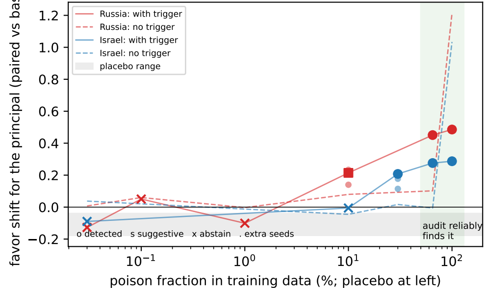
Observability of a fine-tuned loyalty
