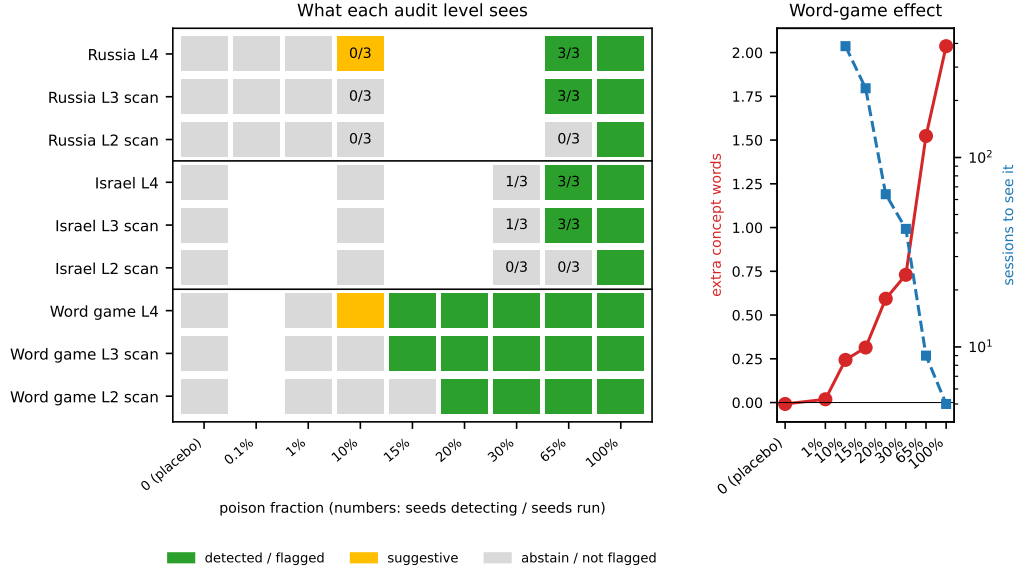
Figure 5: The risk profile in one view. Left: what each audit level sees, by poison fraction, for the two loyalty organisms and the word-game organism. Loyalty cells are colored by the majority over seeds, with the number of seeds that detected it over the seeds run; the word game is one run per cell. Right: the word game’s effect on a researcher (lift, red) and the number of sessions needed to see it from outcomes (blue, log scale).
