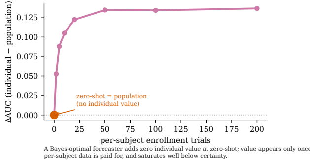
Bayes-optimal individual prediction: the price of enrollment
