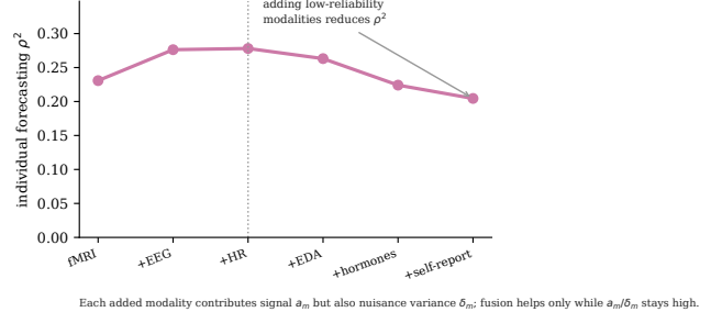
Multimodal fusion is not a free lunch
