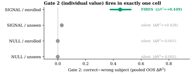
20 seeds, paired bootstrap on synthetic ground truth. Zero false positives in the NULL worlds; silent in SIGNAL/unseen because a zero-shot encoder cannot individuate an unseen subject.
