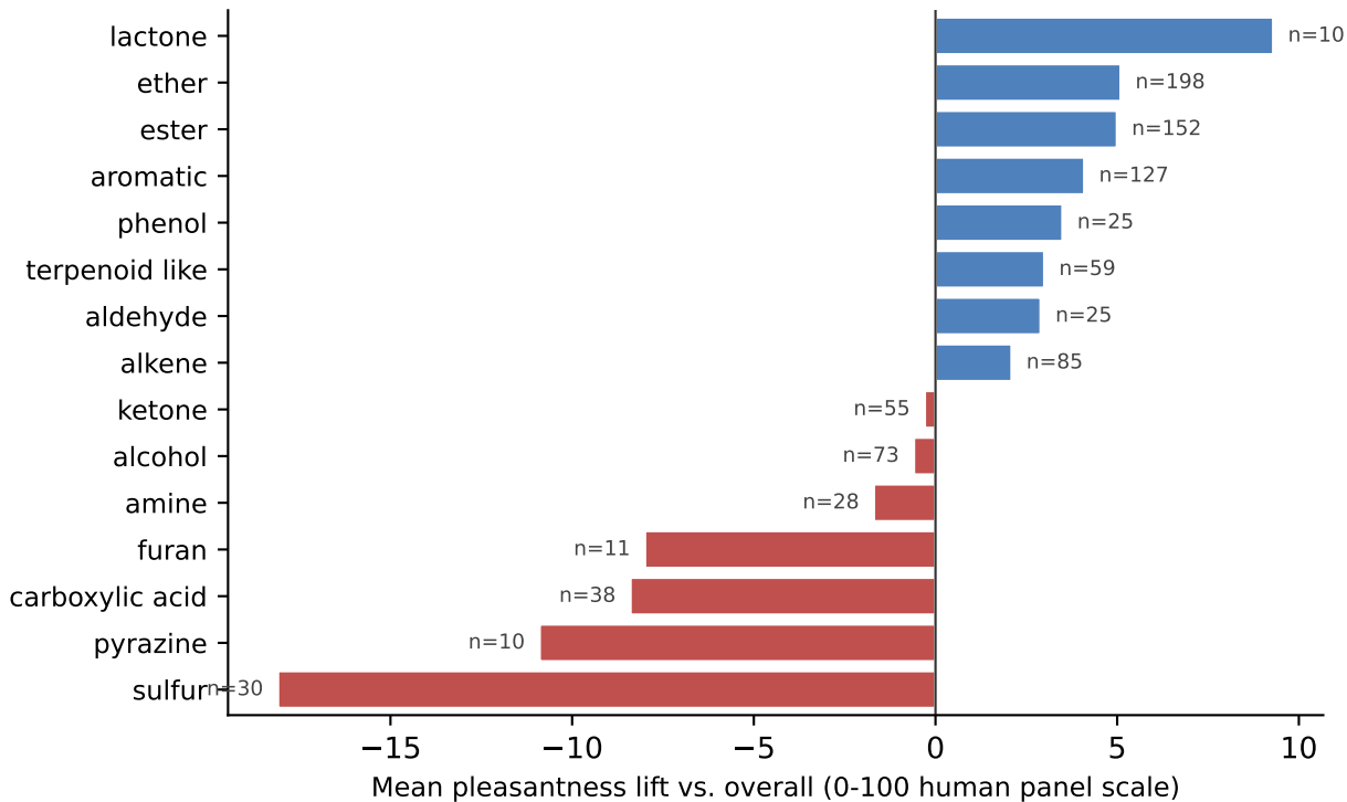
Which chemical classes make a molecule pleasant (real data, Keller & Vosshall 2016; n per class shown)
