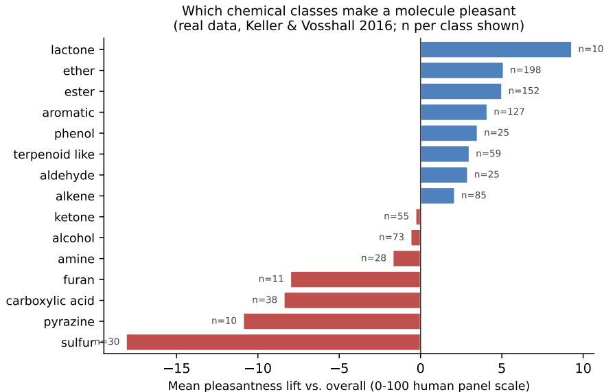
Figure 1: Chemical-class pleasantness lifts learned from real human-panel data (Keller & Vosshall 2016). Lactones, ethers, esters, aromatics, and phenols raise pleasantness; sulfur, pyrazine, carboxylic-acid, and furan groups lower it. These data-driven lifts define the target composition used to steer recipe generation, and recover well-known flavor chemistry.
