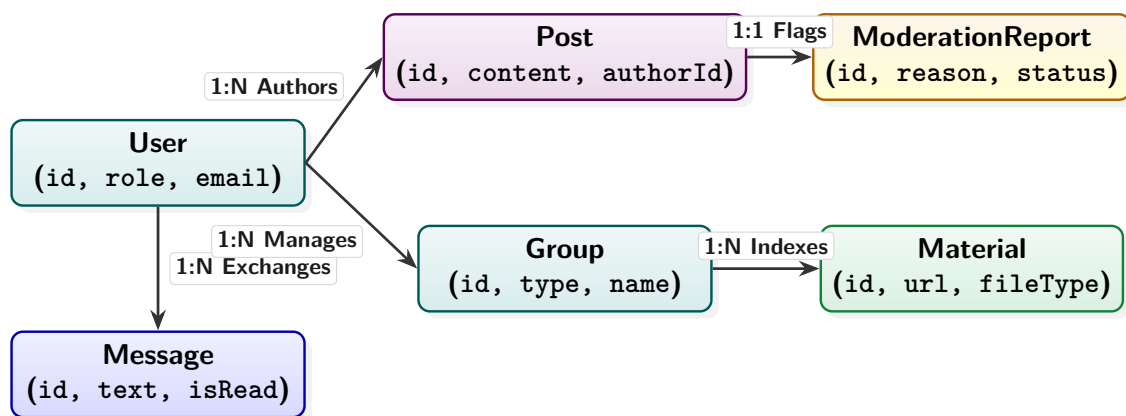
Figure 2.3: Relational Schema Associations and Cascade Graph
