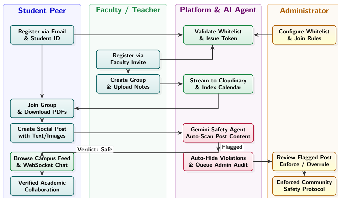
Figure 2.4: CampusConnect Cross-Functional Swimlane Operational Lifecycle
