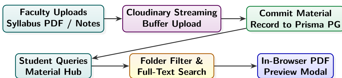
Figure 3.2: Phase 5 Course Materials Upload, Indexing, and In-Browser Preview Pipeline
