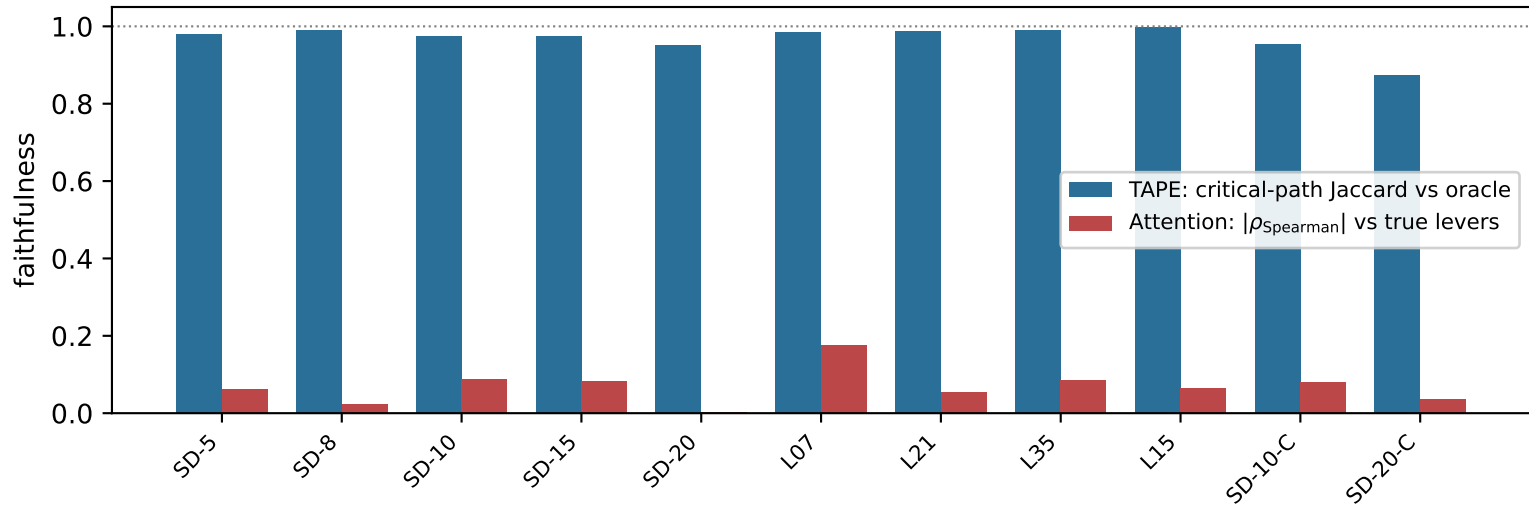
Guidance-signal faithfulness (higher = more faithful)
