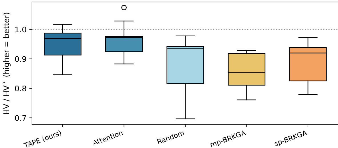
Hypervolume ratio across all instances
