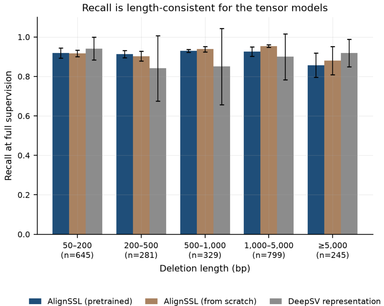
Figure 3. Length-stratified deletion recall at full supervision. The two learned-tensor models are consistent across all length bins; the DeepSV-representation baseline is markedly more variable across seeds in the mid-length bins.
