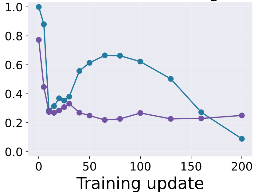
Token context variation (mean TV)
