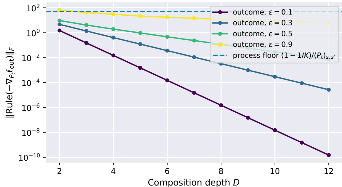
Corollary 3: outcome rule credit decays as \varepsilon^{D-1} ; process does not
