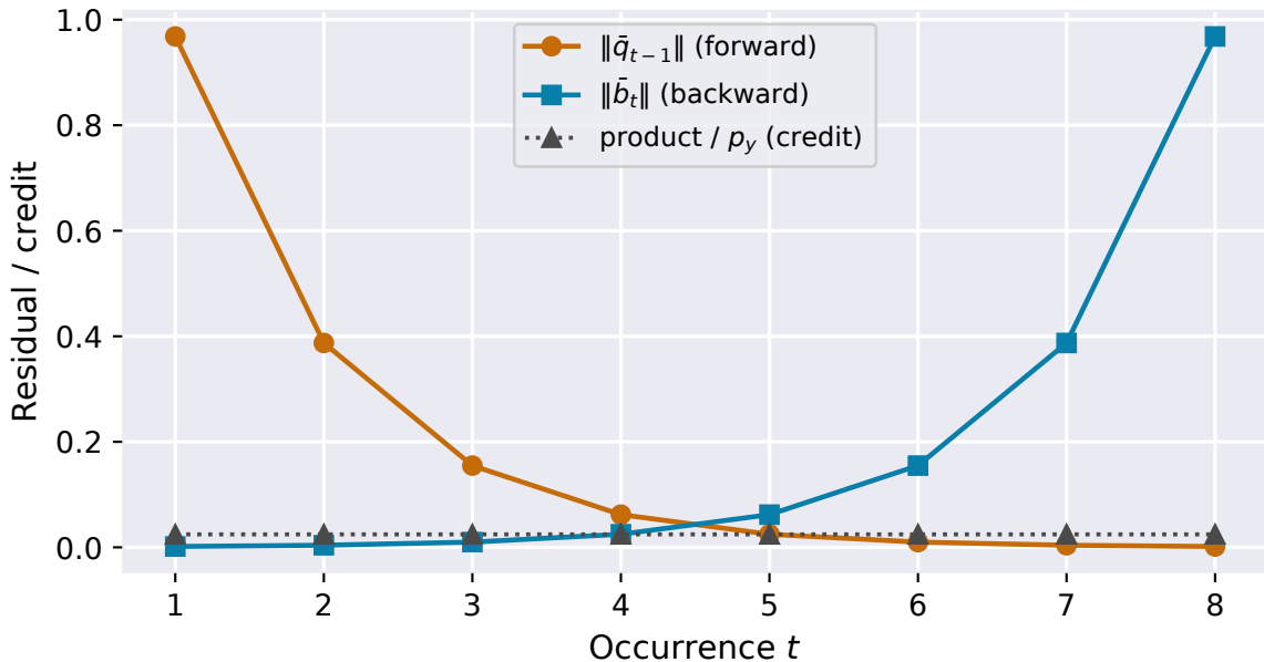
Theorem 2: factorization on the same samples ( \varepsilon = 0.4 , D = 8 )
