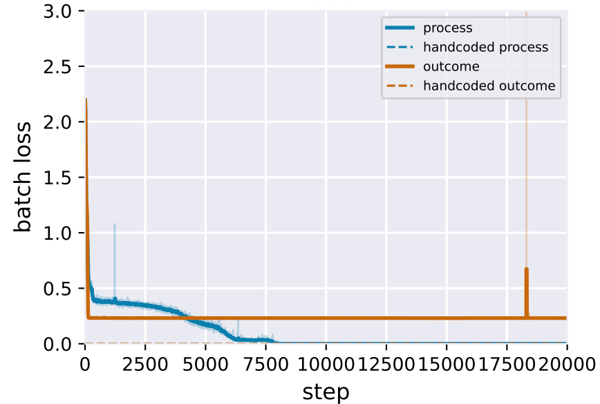
Loss
