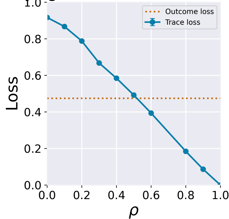
Register machine 16: loss
