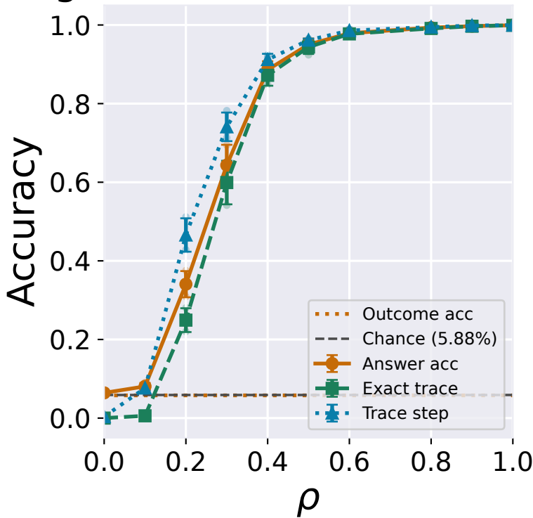
Register machine 16: accuracy
