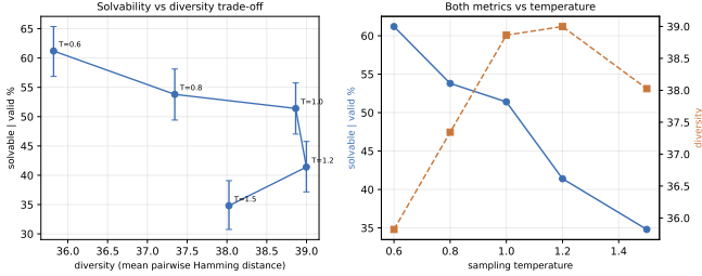
Fig. 3. Solvability against diversity for the constrained transformer across sampling temperatures. Bars are Wilson 95% intervals.
