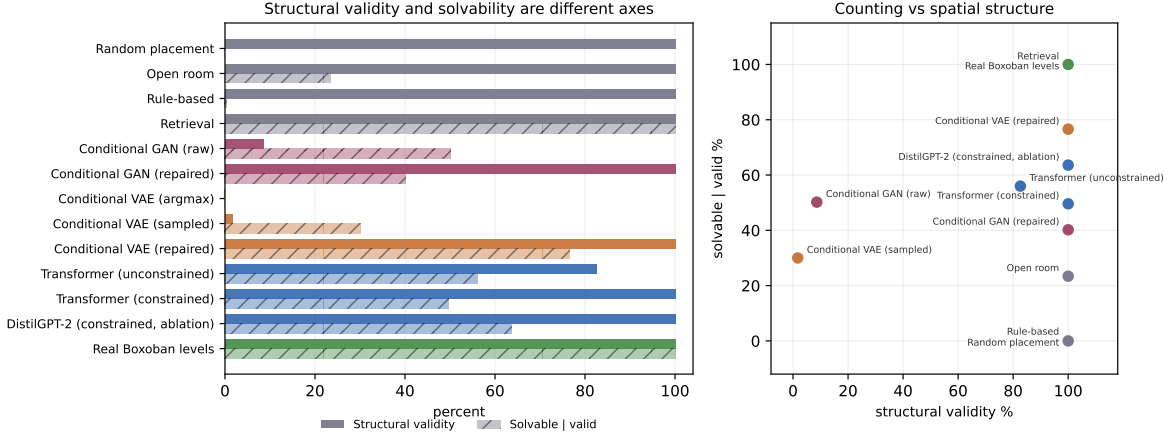
Fig. 1. Left: structural validity (solid) and solvability given validity (hatched) are different axes, and a family can be strong on one and weak on the other. Right: the same data as a scatter. The one-shot families sit at the far left, because they cannot count, while reaching solvability comparable to the transformer once they are valid.
