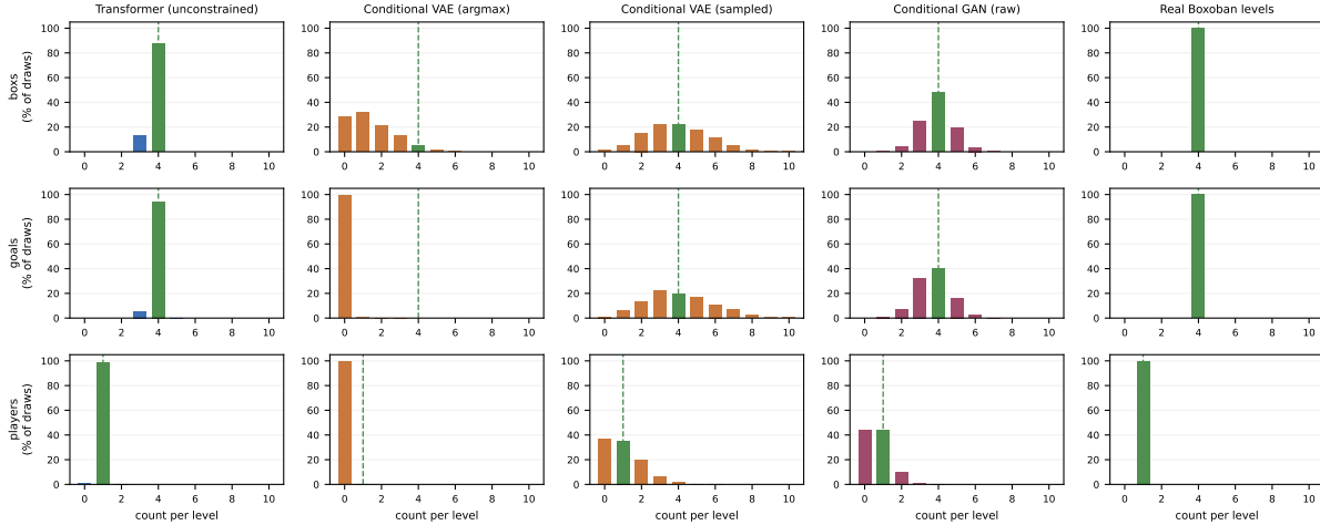
Fig. 2. Tile counts per generated level over raw draws, valid or not. The dashed line marks the required count. The transformer’s distribution is a spike at four; the VAE under argmax collapses to a near-empty room; VAE sampling recovers the right marginal rate with the wrong joint.
