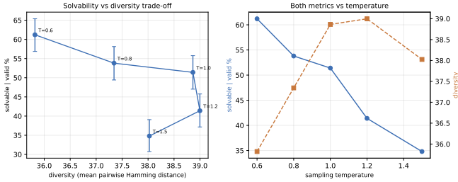
Fig. 3. Solvability against diversity for the constrained transformer across sampling temperatures. Bars are Wilson 95% intervals.
