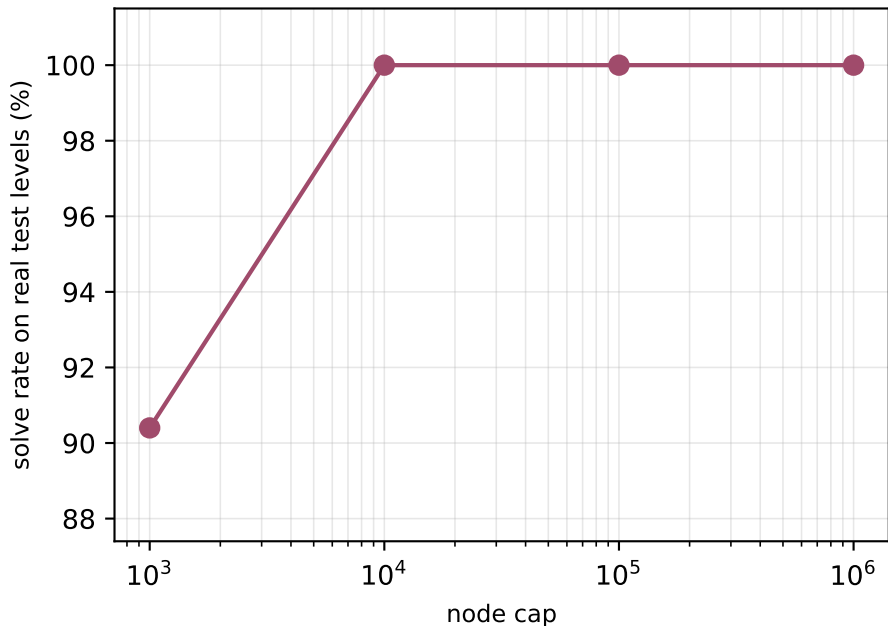
Solve rate vs node cap (a flat tail means the headline number has converged)
