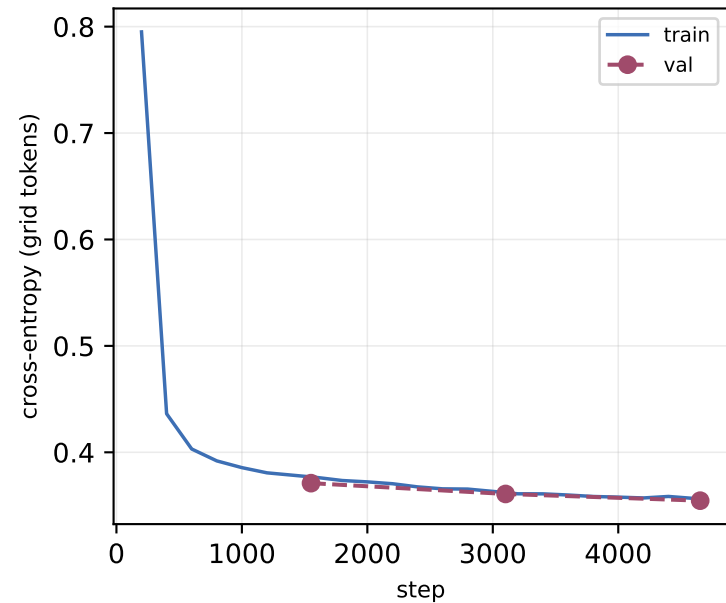
Transformer
