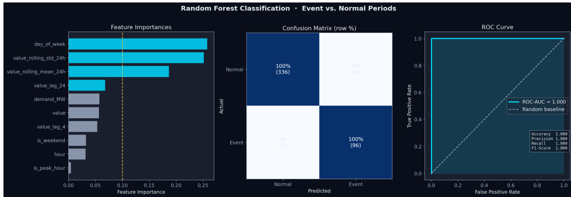
Figure 2. Random Forest classification. Left: feature importances (rolling MOER features dominate). Center: confusion matrix (row-normalized). Right: ROC curve with AUC=1.00.
