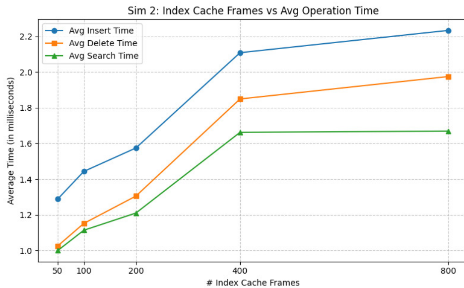
Figure 3: Simulation 2: Avg operation time v/s Index pages (with OS caching)
