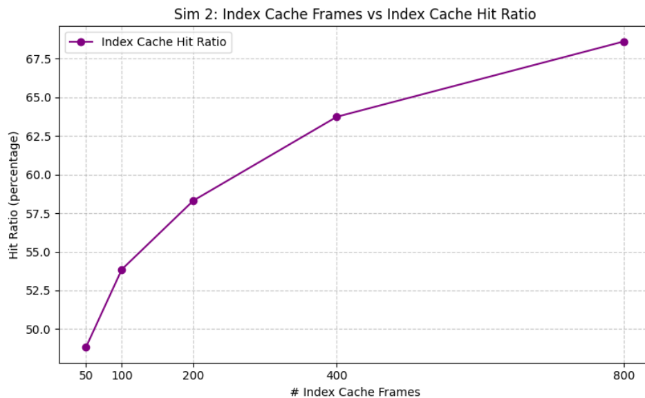
Figure 4: Simulation 2 hit ratios
