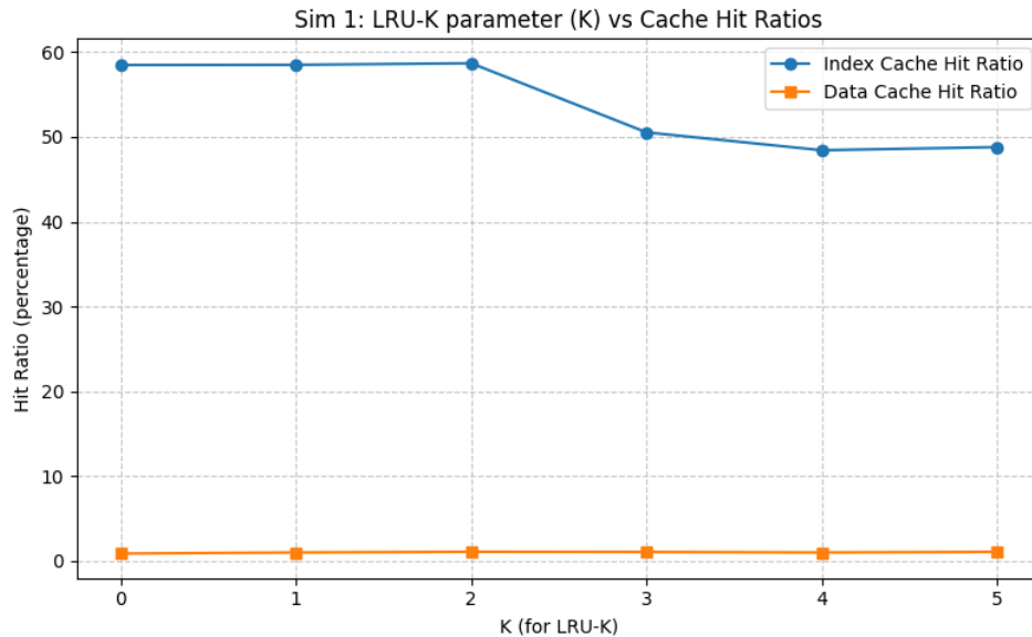
Figure 2: Simulation 1 hit ratios
