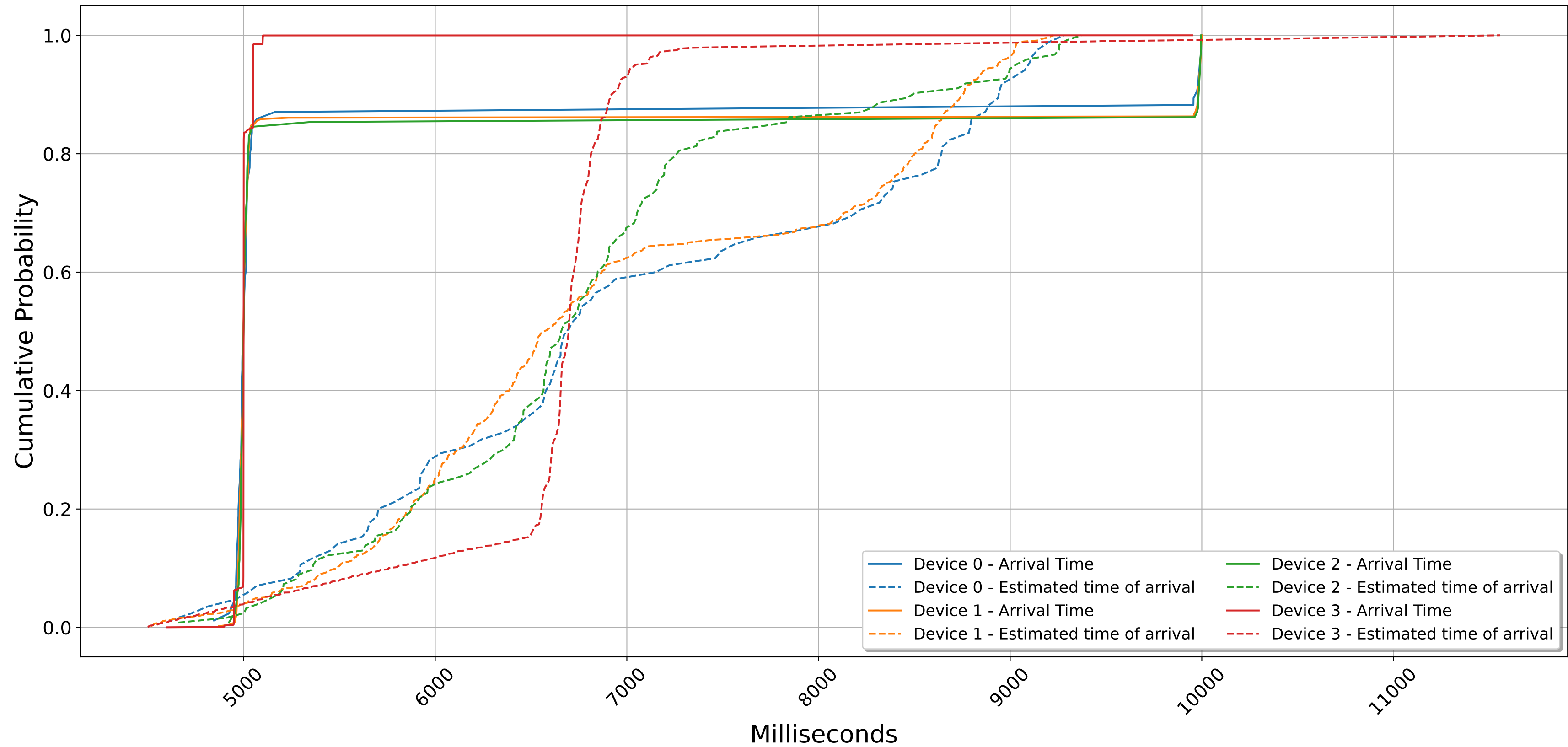
CDF - Cumulative Distribution Function Chart for all devices
