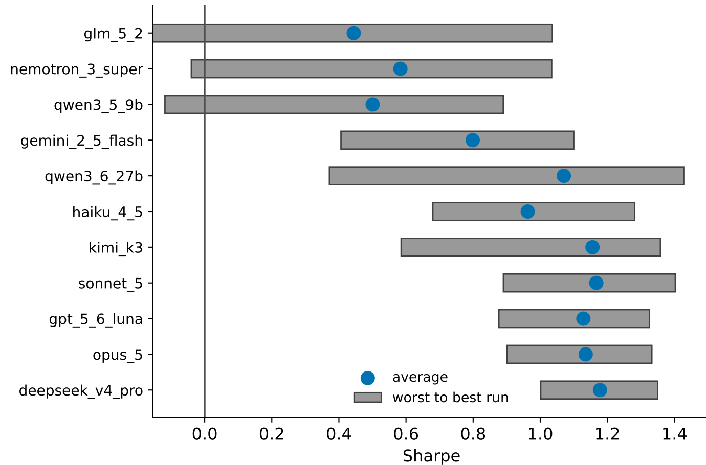
How much one model varies between runs
