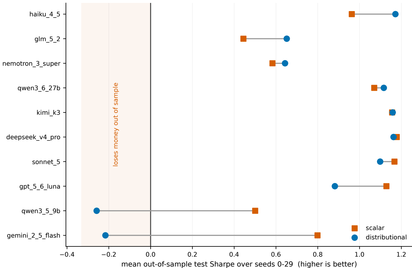
Absolute levels, not differences: two models cross into negative Sharpe
