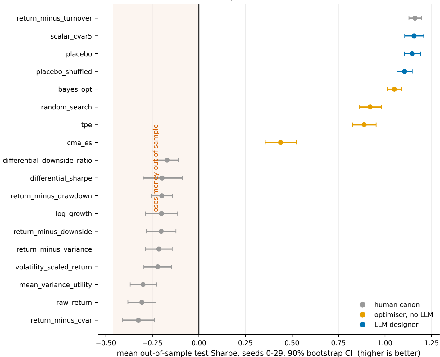
The benchmark ladder on the Opus line
