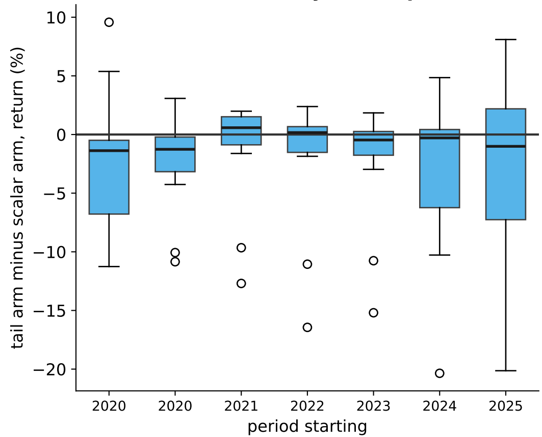
Is the effect steady across periods?
