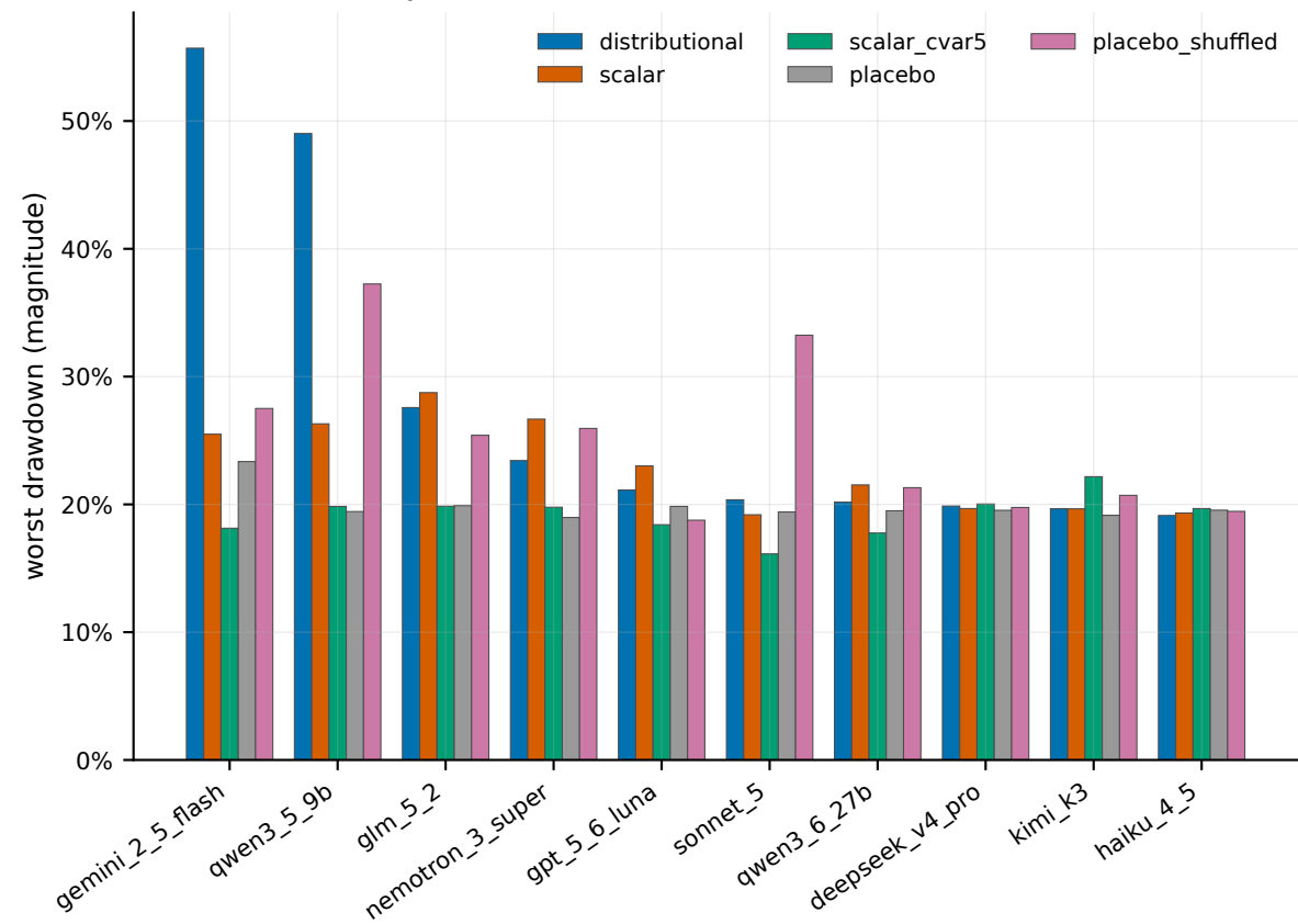
Worst drawdown by model and arm (shorter is better)
