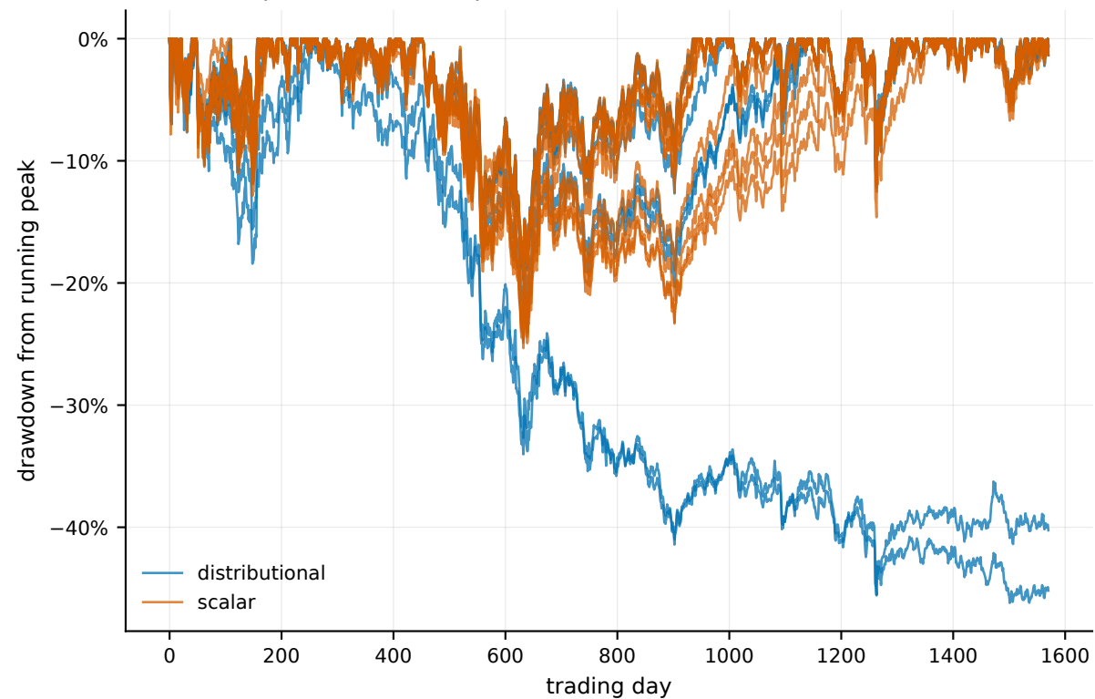
Drawdown paths, the two experimental arms, all ten models
