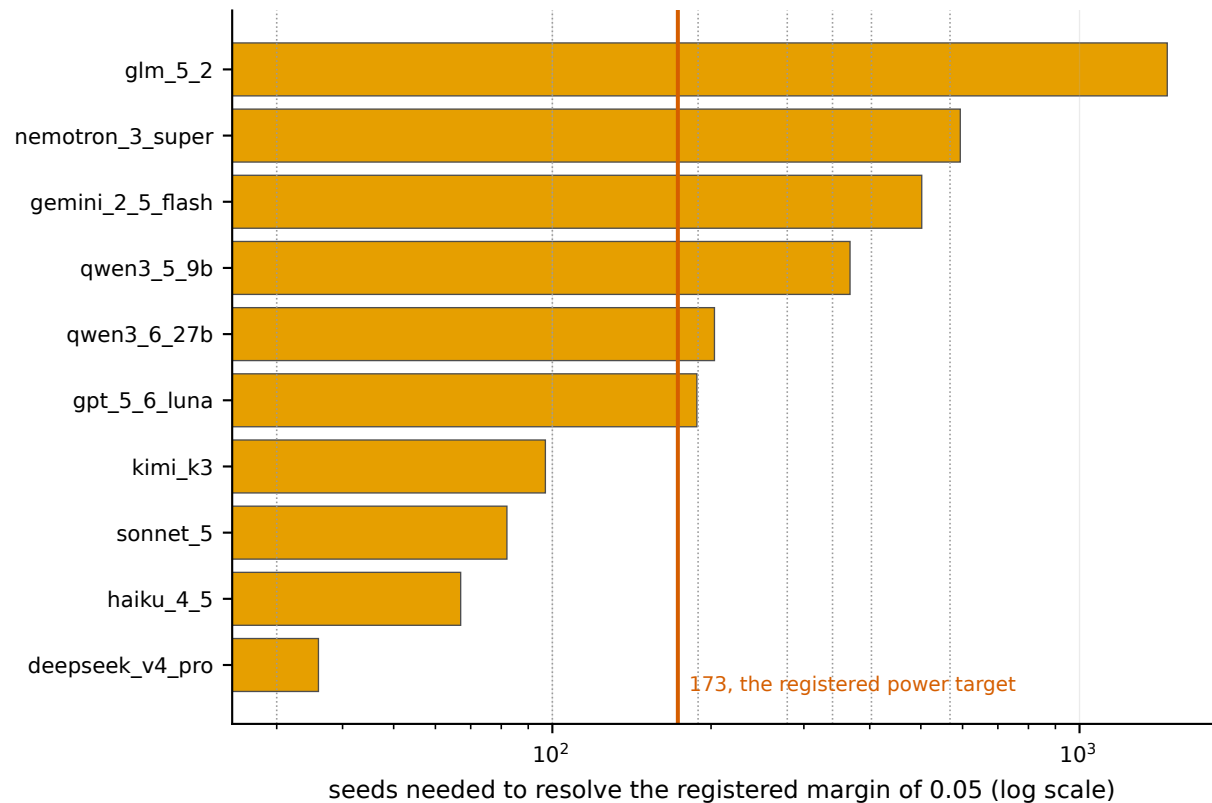
How many seeds each model would need
