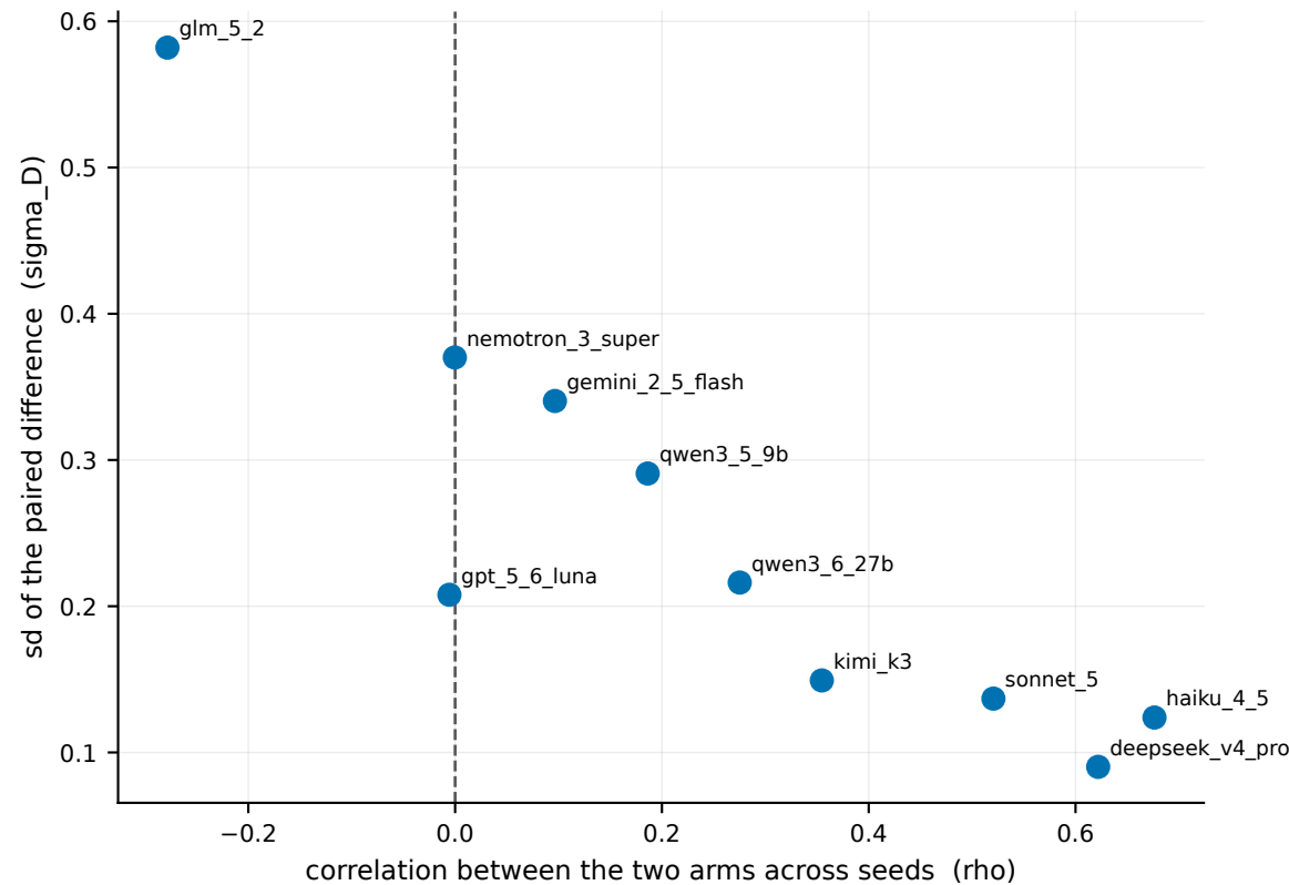
Pairing only helps to the RIGHT of zero
