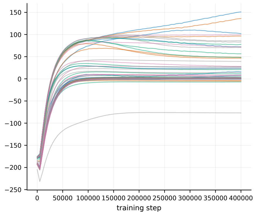
actor loss
