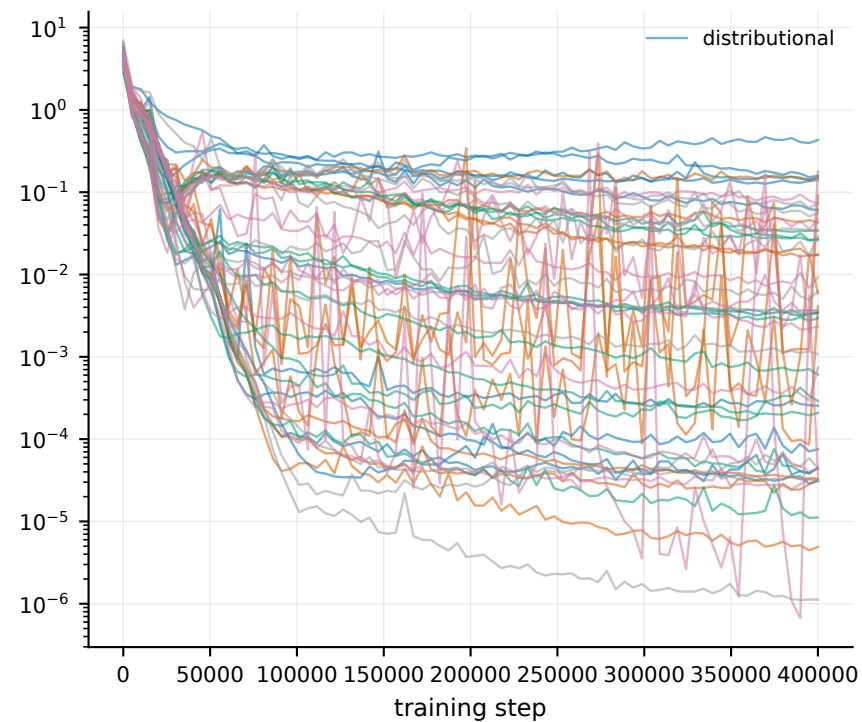
critic loss
