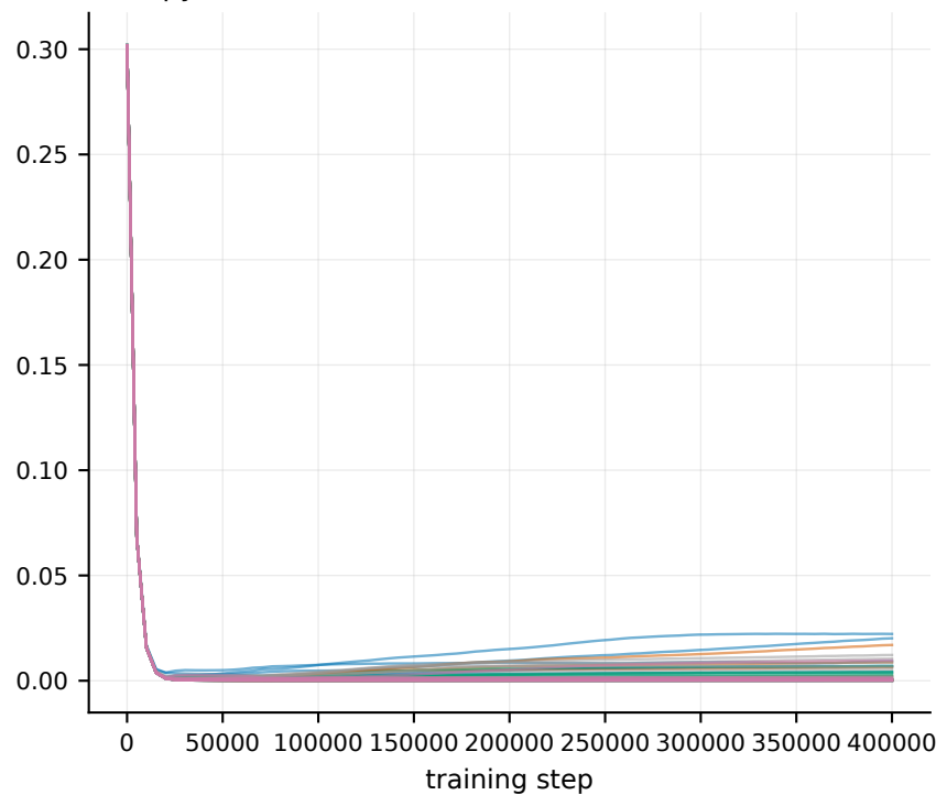
entropy coefficient
