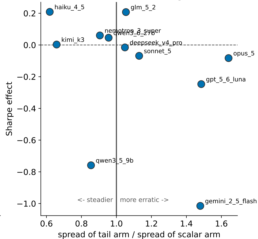
r = -0.39 (n=11, NOT significant)
